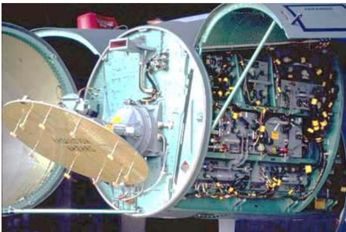
AN/APG-70 F-15C/D/E
