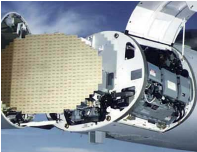
AN/APG-68 F-16C/D
